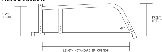
Frame Dimensions
