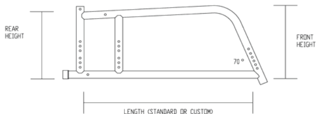
Frame Dimensions
